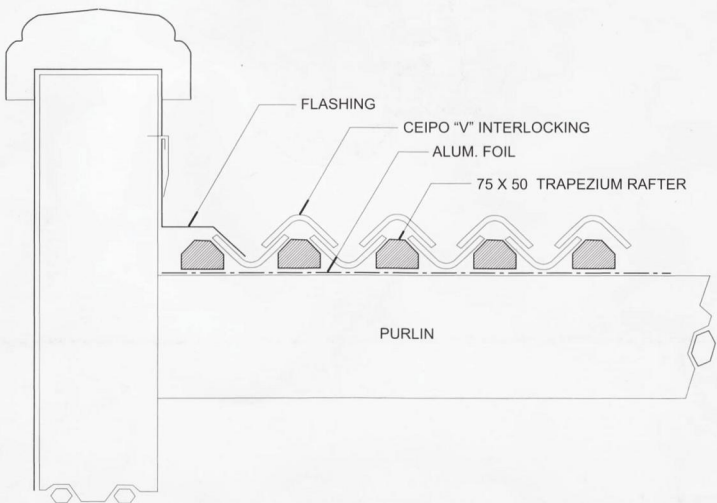
CEIPO "V" INTERLOCKING CLAY ROOFTILES OF ITALY ON TRAPEZIUM RAFTER
