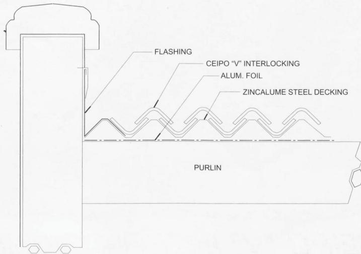
CEIPO "V" INTERLOCKING CLAY ROOFTILES OF ITALY ON METAL DECKING
